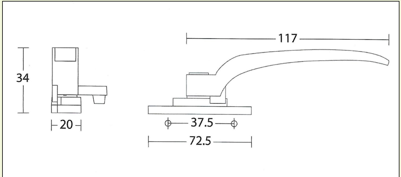
Figure 1: C063(V2) Casement Window Handle (L/R)
