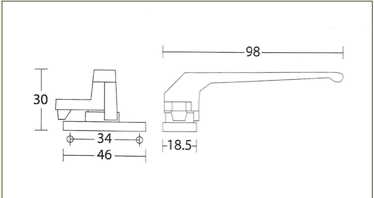
Figure 1: 061 Casement Window Handle (L/R)
